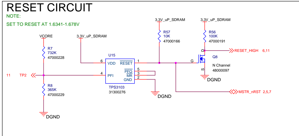
Figure 3.1: Reset Circuit
